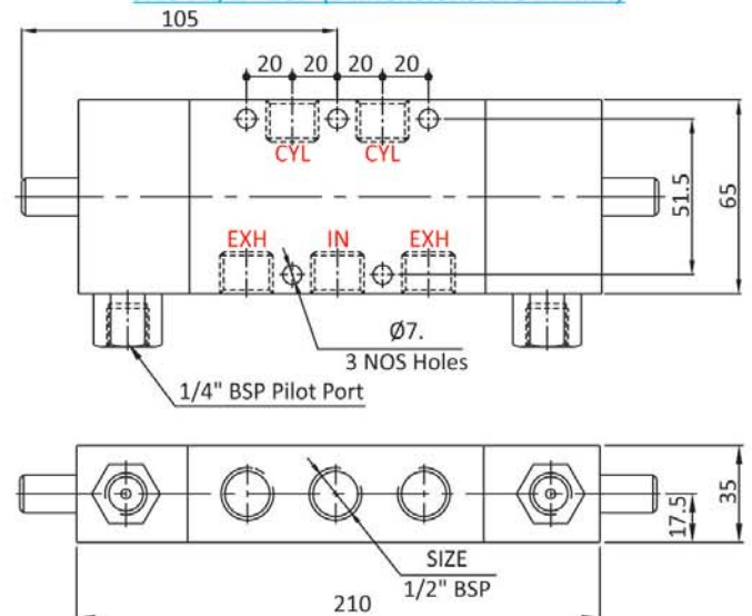
Size : 1/2" BSP (Dimensions are in mm)
